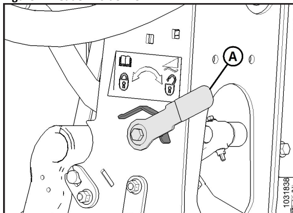
Figure 2: Float Unlocked – Left Side
