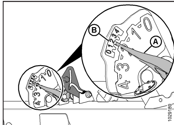
Figure 4: Checking Float – Left Rear View
