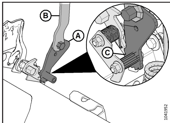
Figure 3: Checking Float – Left Rear View
