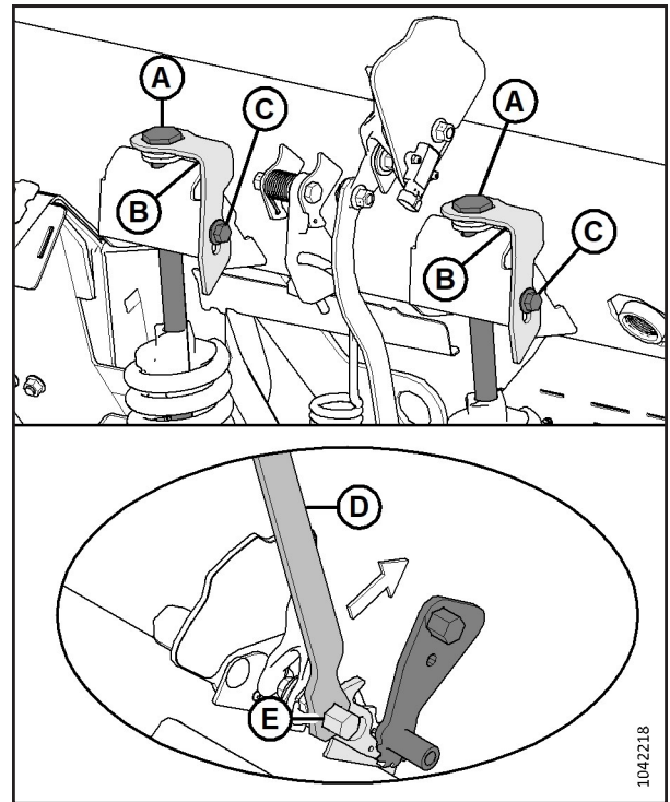
Figure 5: Float Adjustment Bolts – Left Side Shown
