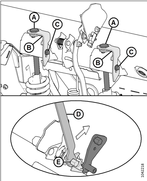
Figure 6: Float Adjustment Bolts and Multi-Tool on Pawl
