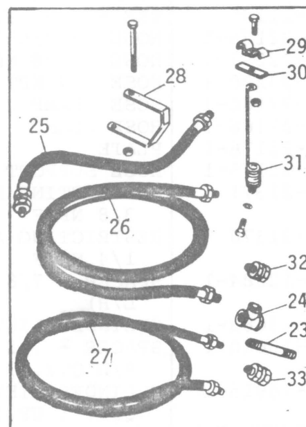
REMOTE-TRACTOR HYDRAULICS
