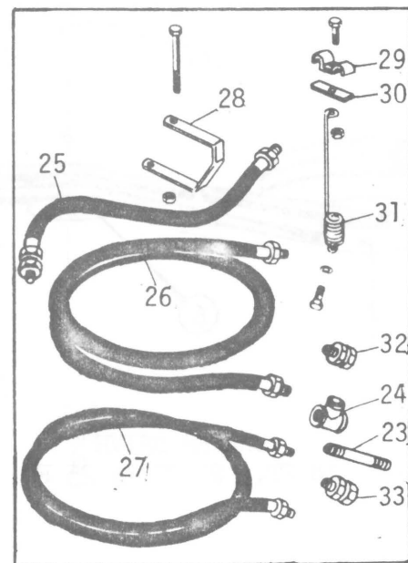
REMOTE-TRACTOR HYDRAULICS
