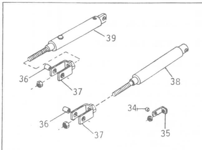
NON-CURRENT CYLINDERS AND BRACKETS
