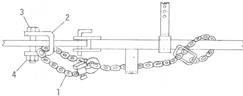
MAIN HITCH
