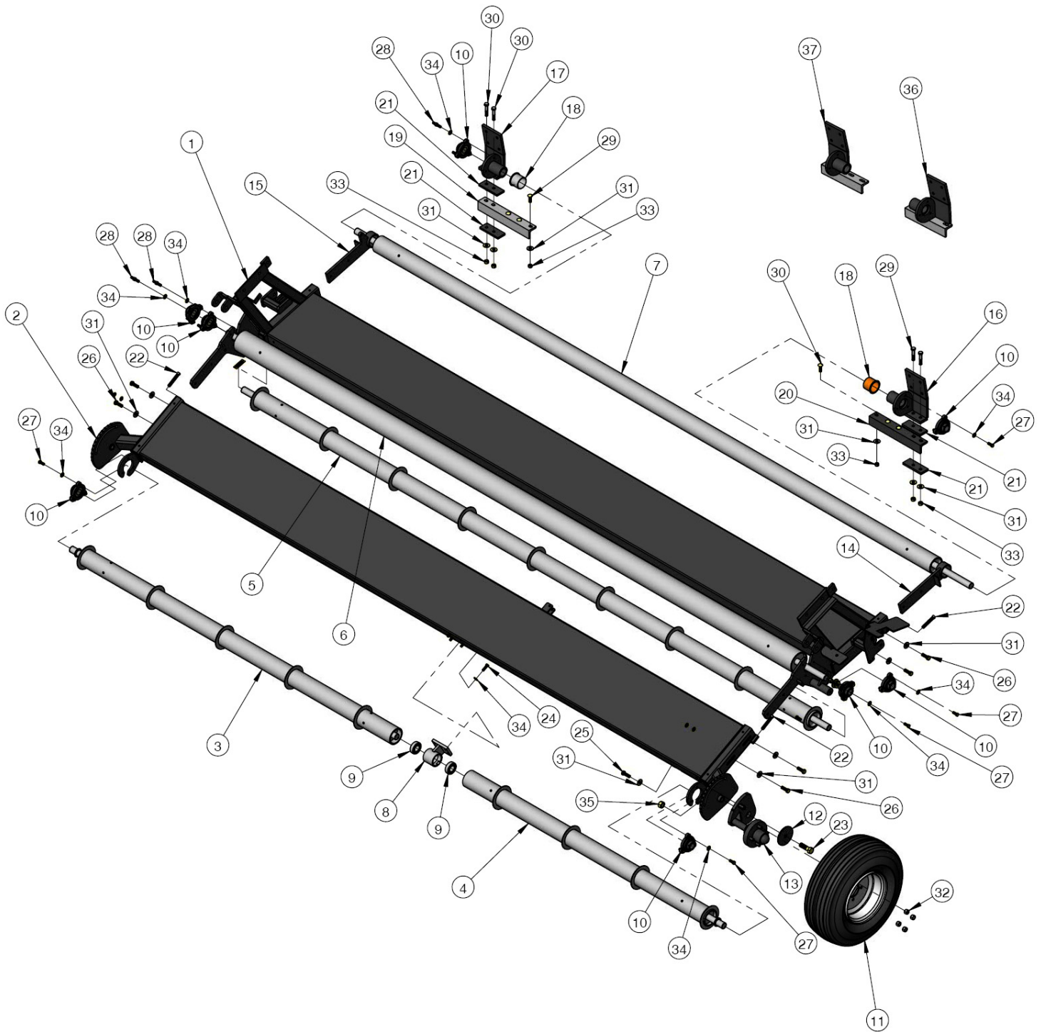
ROLLER, TIRE FRAME ASSEMBLY
