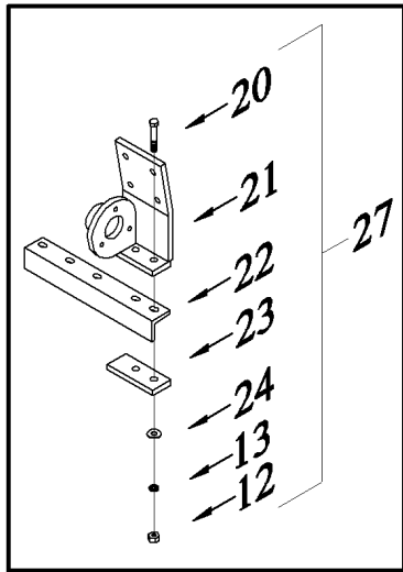
14' & 16' MOUNTING BRACKET
