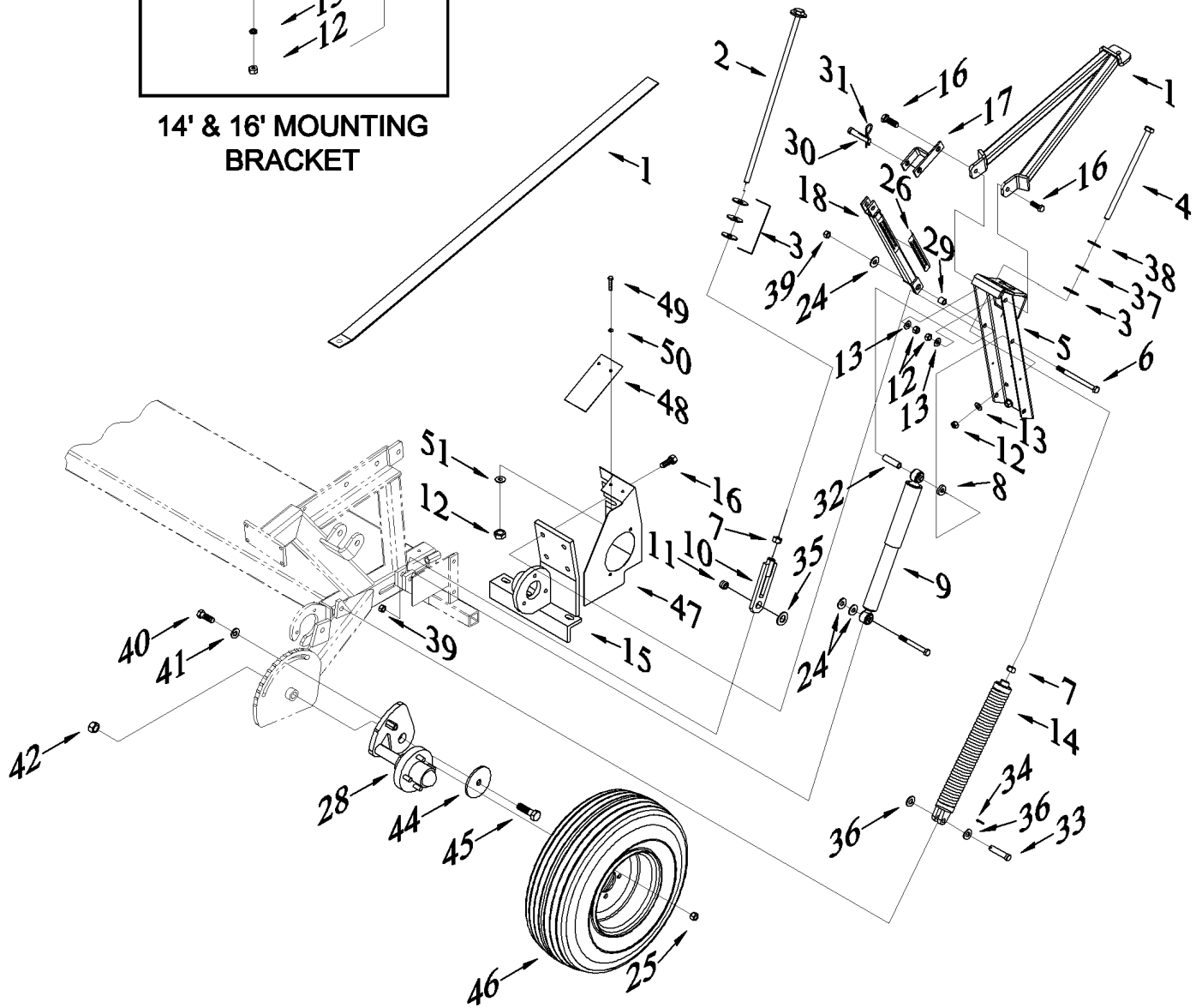
MAIN FRAME MOUNTING ASSEMBLY
