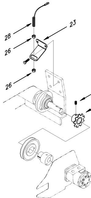
RAKE-UP STANDARD MODEL
