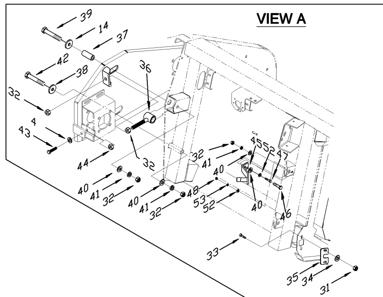
AUGER DRIVE &amp; SUPPORT (LH)
