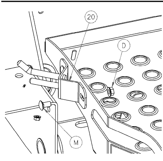
LH PLATFORM REMOVED FOR CLARITY
