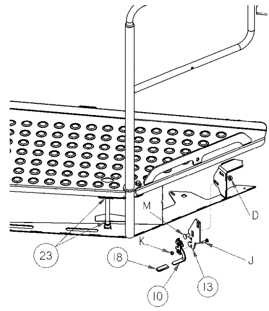
LH PLATFORM SHOWN
