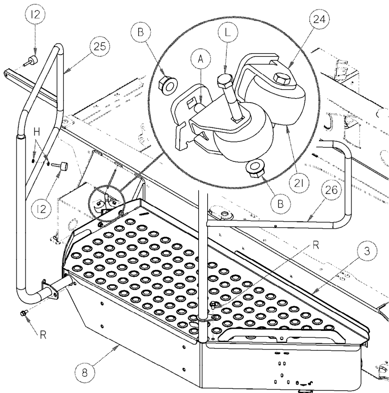
LH PLATFORM SHOWN
