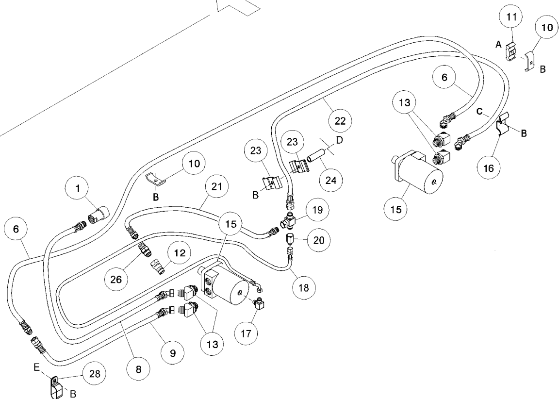
MOTORS OUTBOARD (COMBINE ASSEMBLY)
