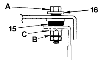
Cab Mounts
