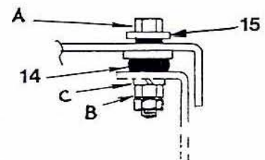
cab mounts
